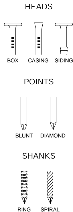
Figure 2: Nail Types
